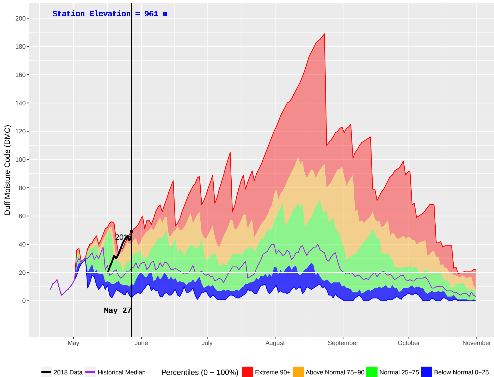
HOLY CROSS 2 (654) : Historical (1998–2016) and Current (2018) Noon Duff Moisture Code (DMC)
